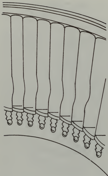
FIGURE 10-60. Turbine blade waviness.
